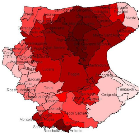
Figure 4. Current PGA for T_R=475 years
