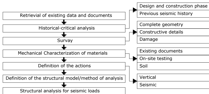
Figure 2. Synopsis of the protocol for the preliminary investigations and the safety assessment.
