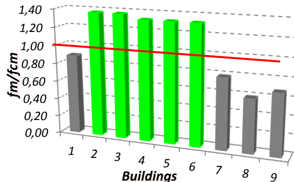
Figure 7. Strength of in-place concrete for the sample compared with the medium value of the design strength f_{cm} = 20.5\text{MPa} (in the normalized scale).
