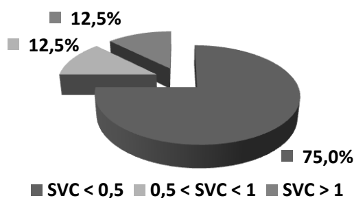
Figure 8. Percentage distribution of the seismic vulnerability of the school buildings expressed as a function of the coefficient SVC.
