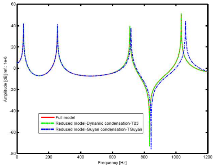
Figure5: FRFs for the full and the reduced systems-Guyan condensation/Dynamic condensation
