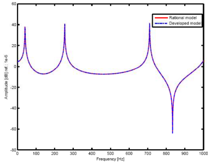
Figure3: FRFs for the rational and the developed GHM model of the viscoelastic sandwich beam The frequency response of the rational model (1) and the developed model (3) are confused. This leads to conclude that these two models are equivalent. They are used as reference in the modeling of the viscoelastic sandwich beam.
