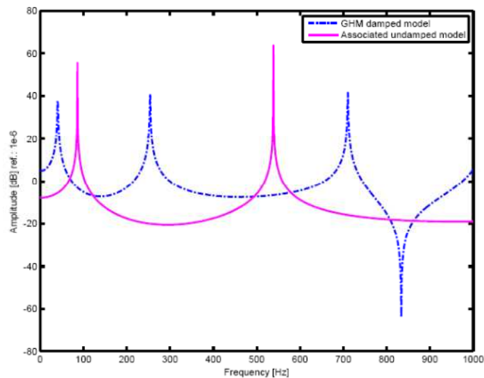
Figure2: FRFs of GHM damped model and his associated undamped model of the viscoelastic sandwich beam
