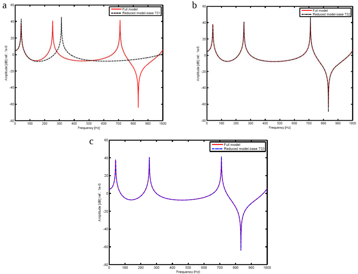
Figure4: FRFs for the full and the reduced systems by using T_{01} (a), T_{02} (b), T_{03} (c)
