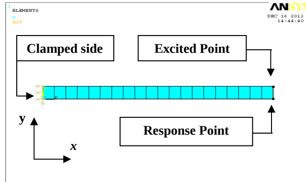
Figure1: Illustration of the FE model implemented for the Clamped-Free (C-F) viscoelastic beam The response of the damped GHM model (described by rational fraction) and his associated undamped model of the beam under a harmonic excitation are presented in figure 2.
