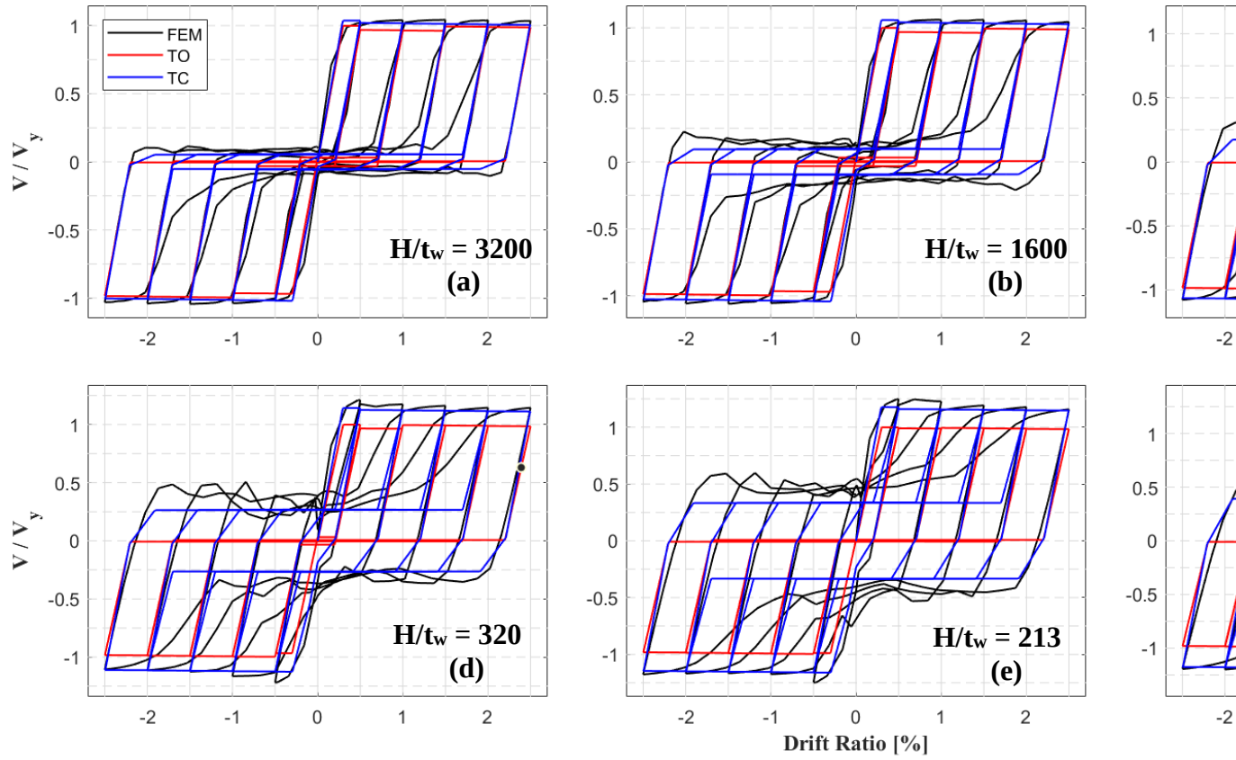
Figure 4: Comparison of normalized base shear vs. drift ratio for an aspect ratio of 1.5
