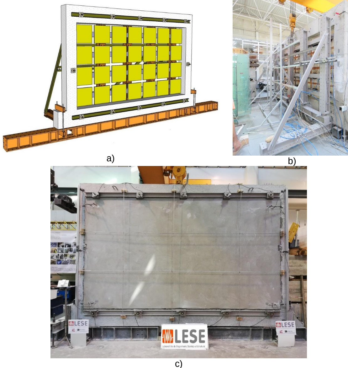
Figure 4: Test setup: a) schematic layout; b) lateral view; and c) front view.
