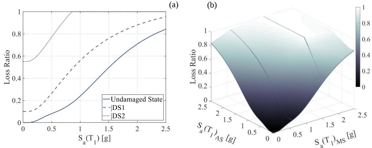
Figure 7. Vulnerability functions for the infilled frame.
