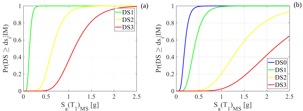
Figure 5. Undamaged state fragility functions for (a) bare and (b) infilled frames.
