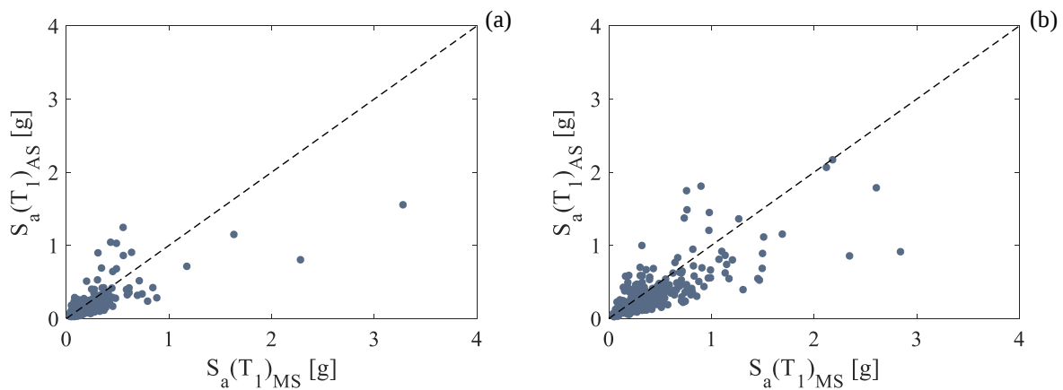
Figure 3. Scatter of S_a(T_1)_{MS} and S_a(T_1)_{AS} for the (a) bare frame and (b) infilled frame.
