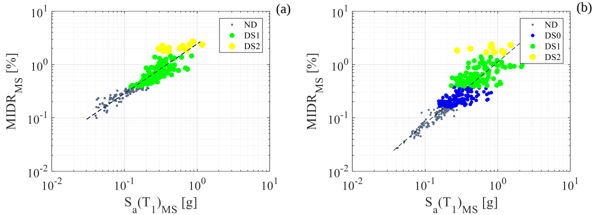
Figure 4. Undamaged state cloud analysis and Probabilistic Seismic Demand Models ( i.e. , S_a(T_1)_{MS} vs. MIDR) for (a) bare and (b) infilled frames.
