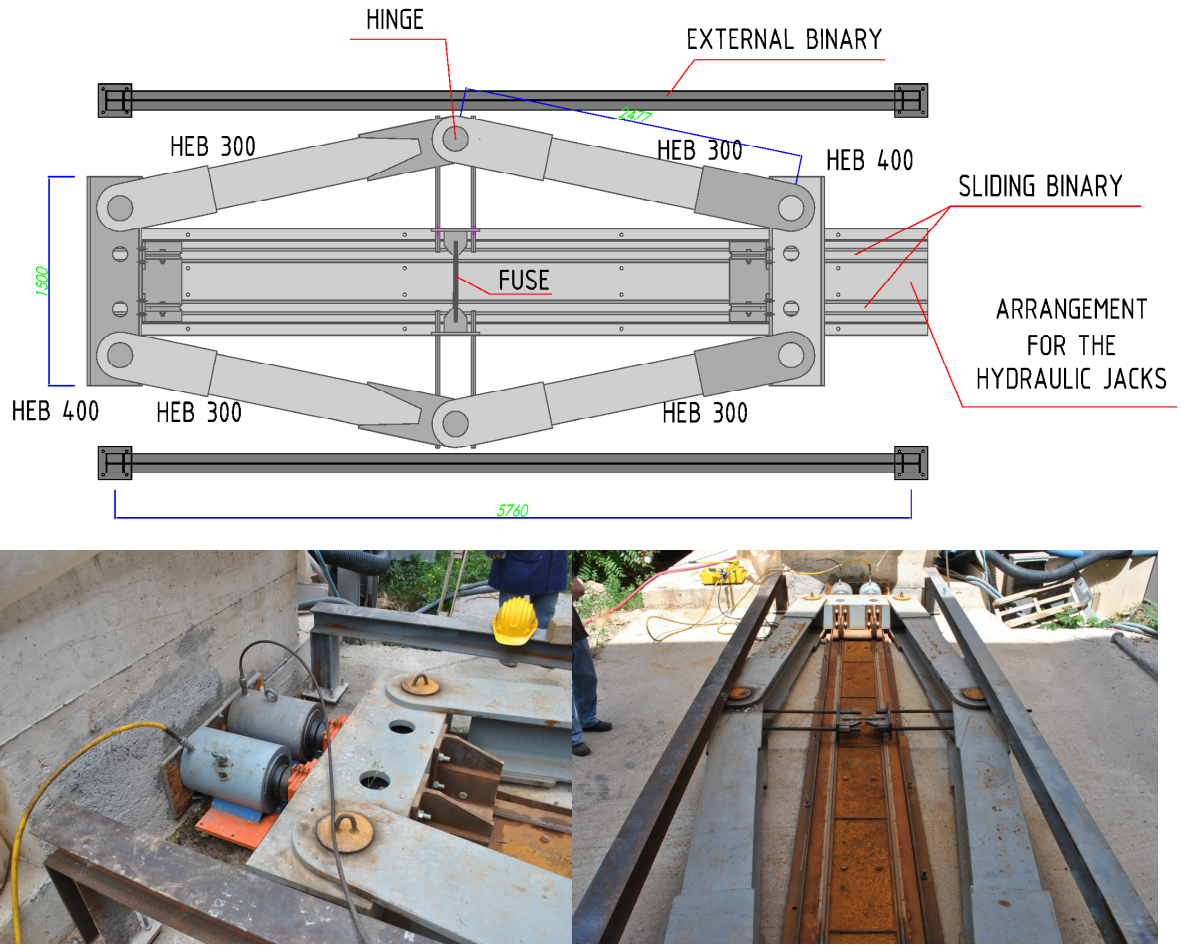
Figure 4: Details of the thrust device.
