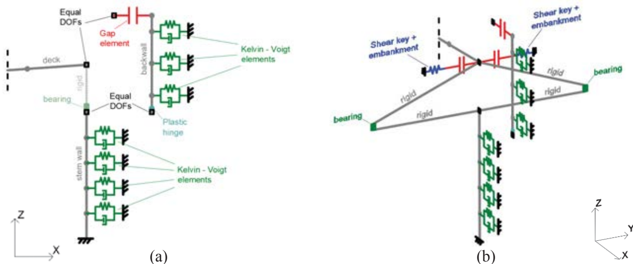
Figure 4: (a) Longitudinal section and (b) 3-d view of the ‘detailed’ abutment-backfill model
