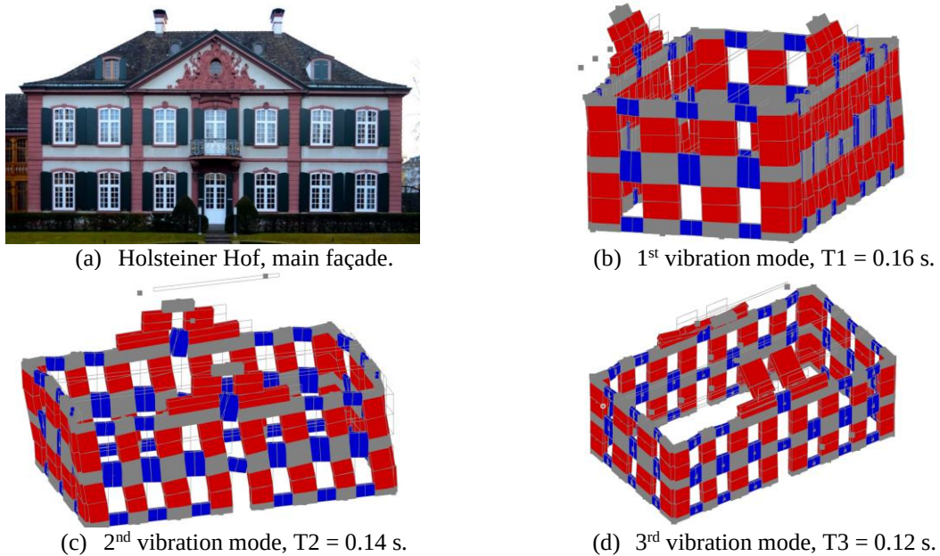
Figure 1. Holsteiner Hof building and numerical model using 3D macroelements.
