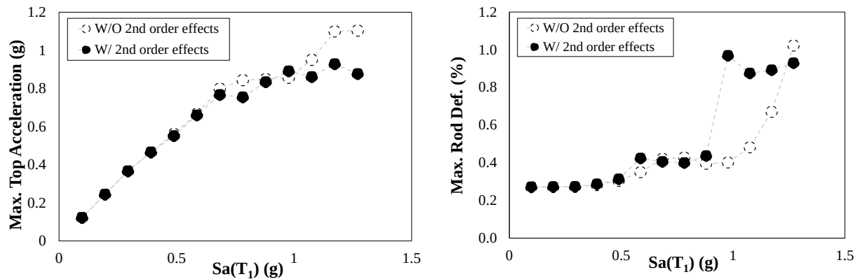
Figure 4: Time-history results (maximum) when second order effects are considered or neglected: displacement at the top, base shear, acceleration at the top and deformation of the PT rods.
