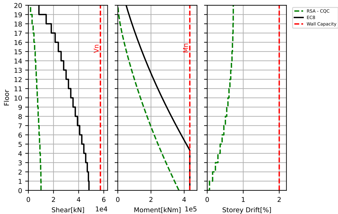
Fig. 3. EC8 capacity design envelope for 20-storey building
