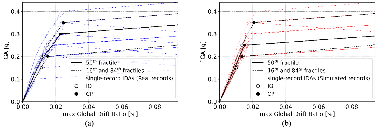
Figure 7: IDA curves displaying maximum values of EDPs for (a) real records and (b) simulated records.
