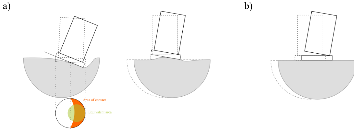
Figure 1: Foundation-structure connection: a) strong enough to cause the partial uplift at the soil-foundation interface and plastic deformation at the soil surface [7]; b) weak enough to cause the uplift of the block at the block-foundation interface [10].
