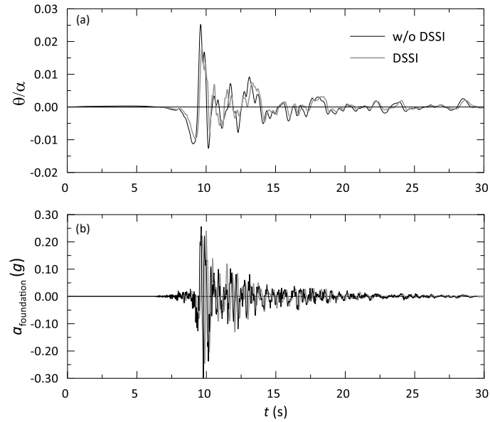
Figure 6: Influence of DSSI on the time histories of the (a) dimensionless rotation block and the (b) foundation acceleration, in the presence of the tie-rod.
