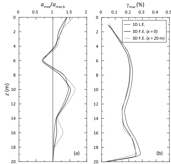
Figure 4: Profiles of the (a) peak acceleration ratio; (b) peak shear strain.
