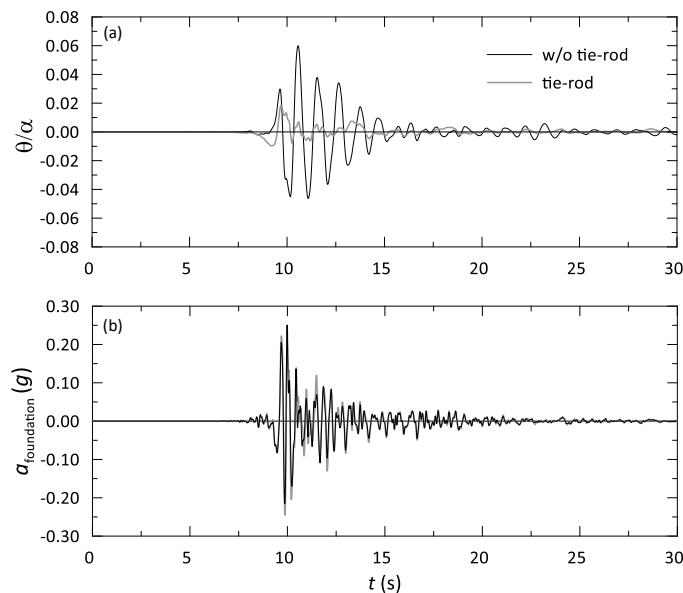
Figure 5: Influence of the tie-rod on the time histories of the (a) dimensionless rotation block and the (b) foundation acceleration, considering DSSI.
