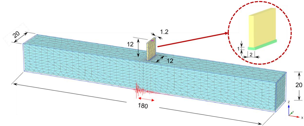
Figure 2: 3D FE model adopted in the time domain numerical analyses (units: m).
