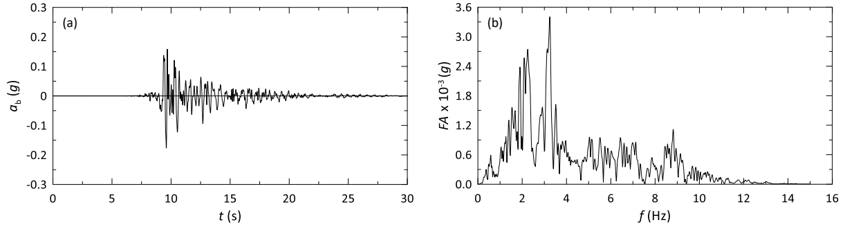
Figure 3: Seismic input adopted in the 3D FE analyses: (a) horizontal acceleration time history; (b) Fourier Amplitude spectrum.
