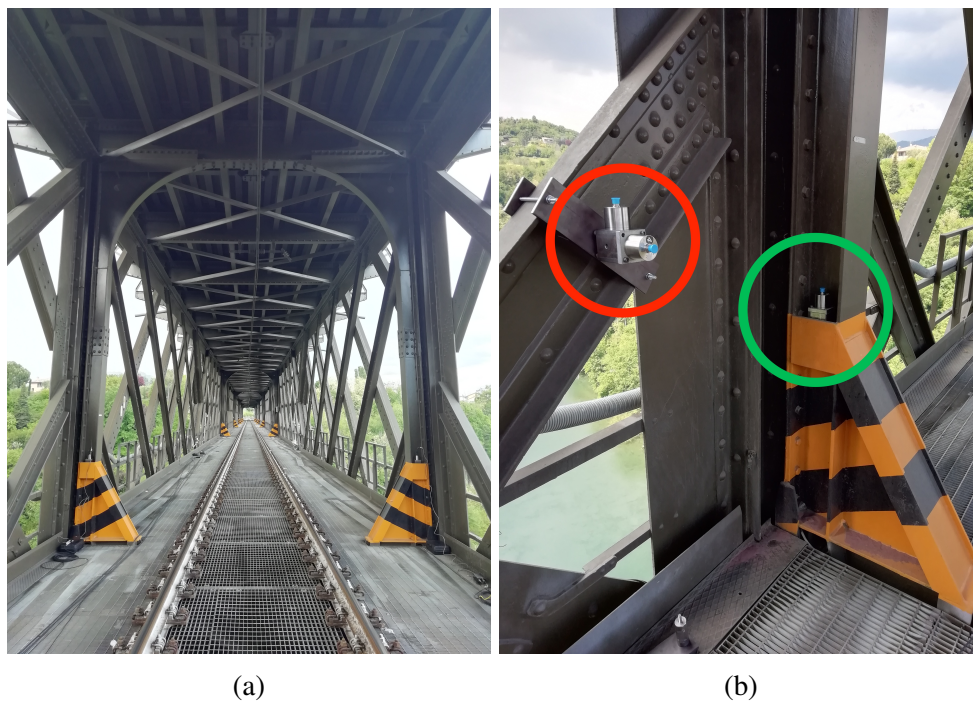
Figure 2: Global inside view of railway deck (a) of San Michele Bridge (1889); typical sensor placements (b).
