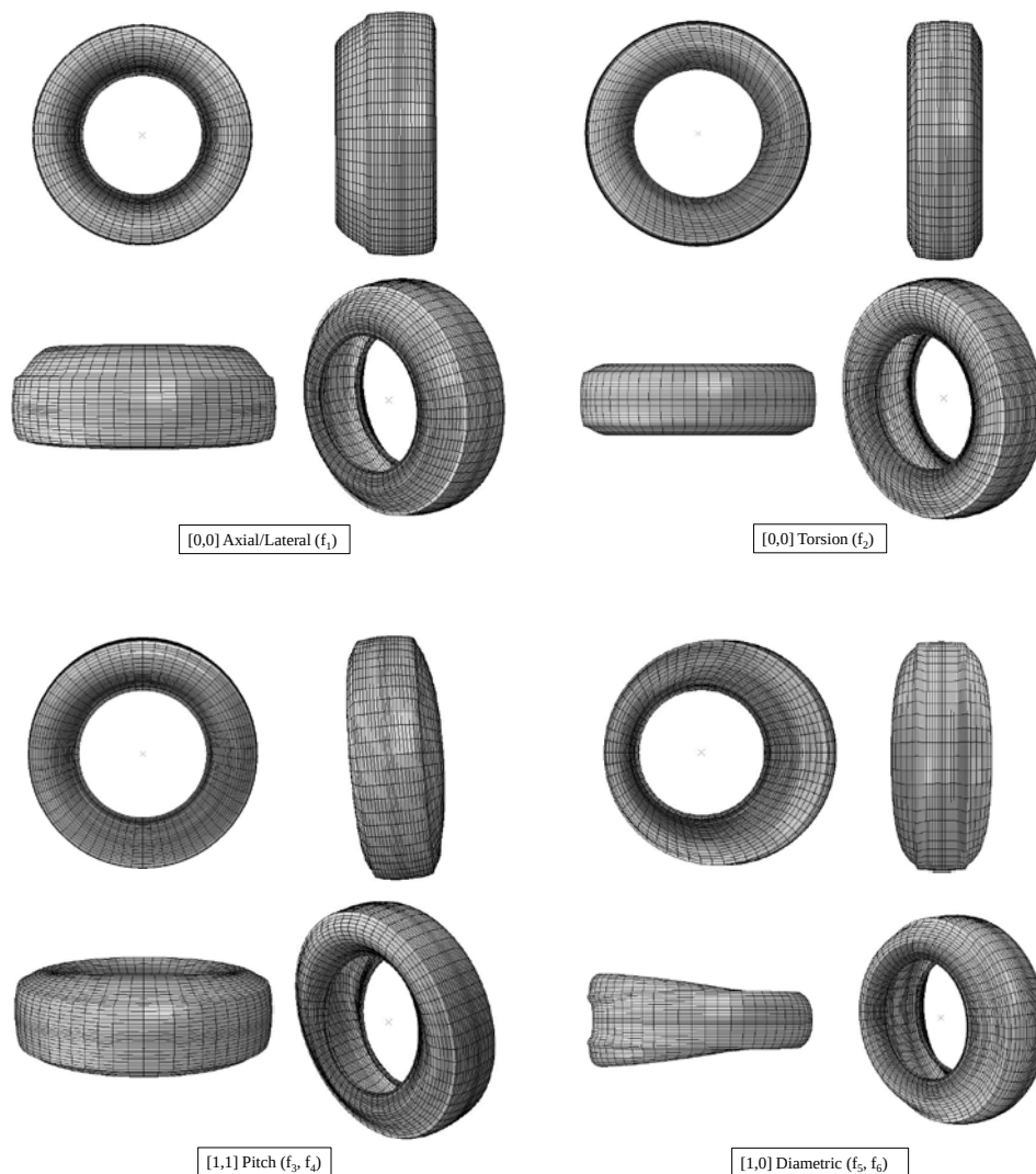
Figure 3: Eigenmode shapes of the optimised tyre model (continued in the next page).
