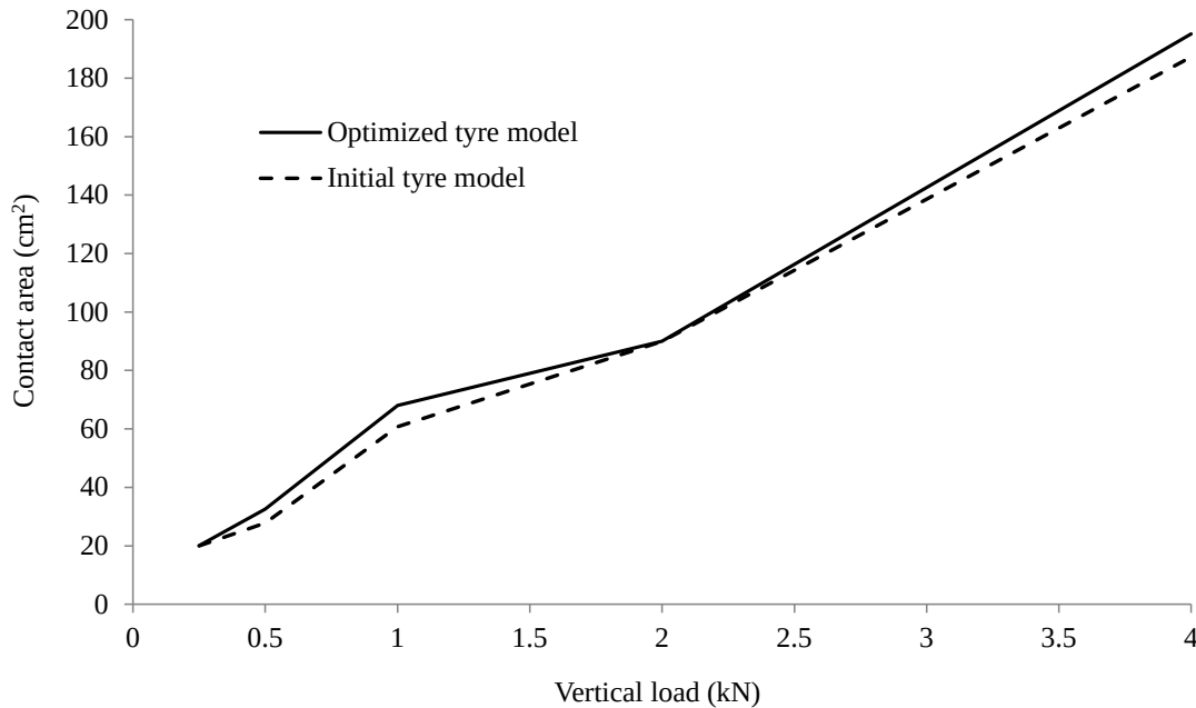
Figure 5: Contact area versus vertical load for the two tyre models considered in this study.
