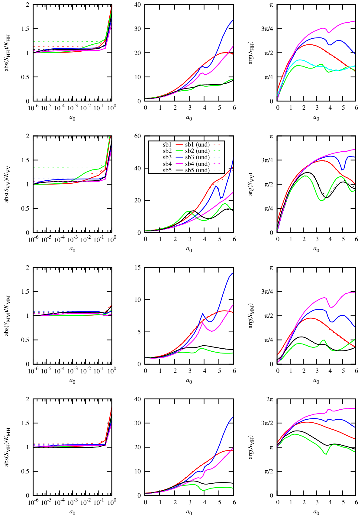
Figure 4: Impedances of bucket foundations with L/D = 1 in proelastic soils and corresponding undrained elastic soils (dashed lines) . From top to bottom: horizontal, vertical, rocking, and horizontal-rocking coupling impedances normalized with respect to the corresponding quasi-static stiffness using the proelastic soil.
