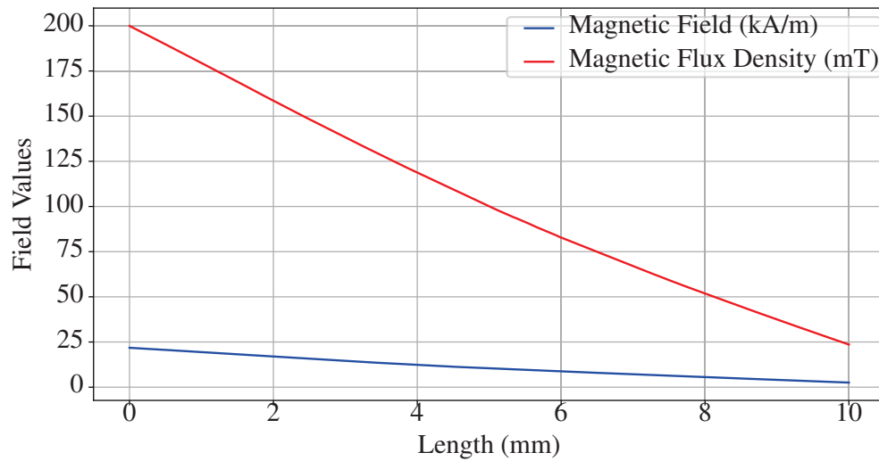
Figure 6: Magnetic field strength in the MRF for TPU wall thickness 0,2 mm
