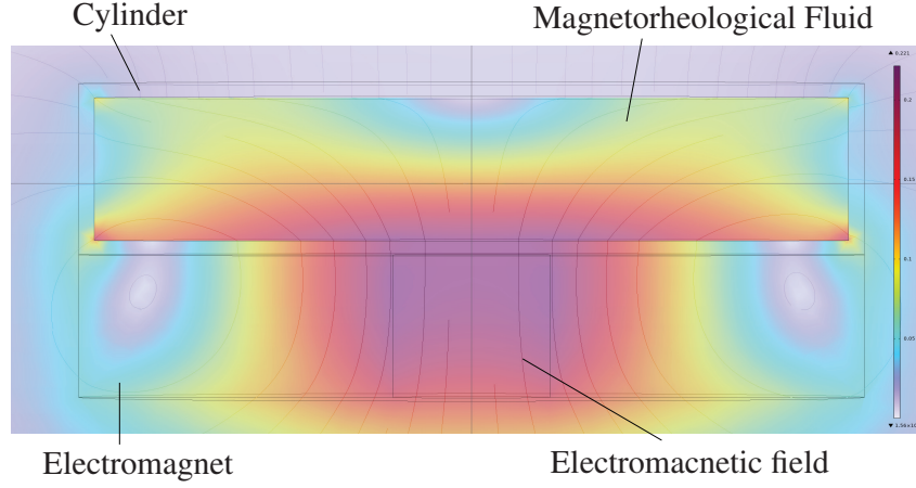
Figure 2: Distribution of the magnetic flux density in an MRF-based setup influenced by an electromagnet. The color scale denotes the magnetic flux density, with red indicating high and blue indicating low field strengths.
