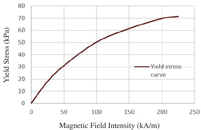
Figure 7: Yield strength vs. magnetic field strength for AMT-RHEOTEC+ MRF
