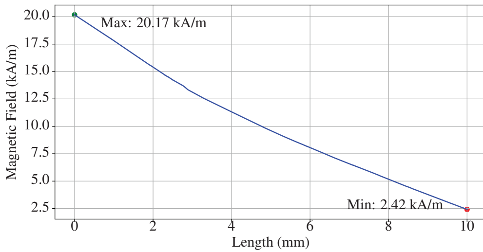
Figure 5: Magnetic field strength in the MRF for TPU wall thickness 1 mm
