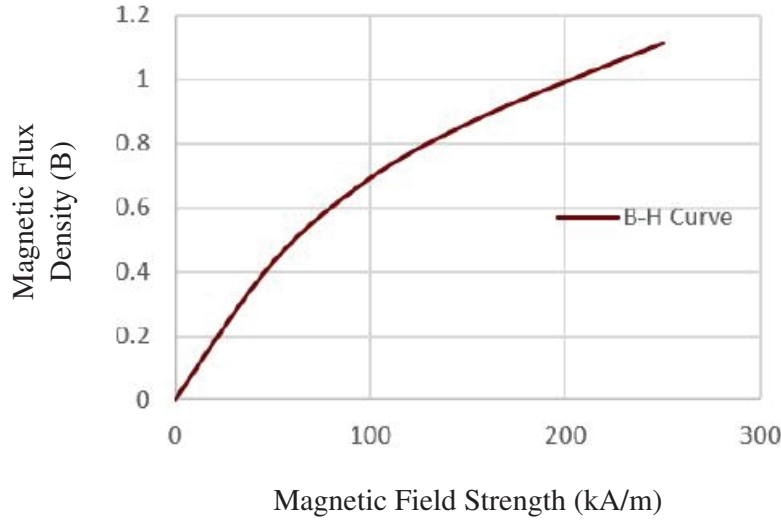
Figure 3: B-H curve for AMT-RHEOTEC+ MRF interpolated in COMSOL
