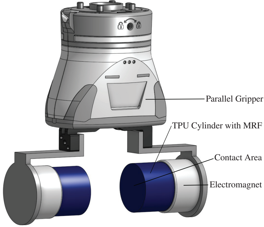
Figure 1: Schematic representation of the underlying gripper concept based on a model sketch using a parallel gripper.
