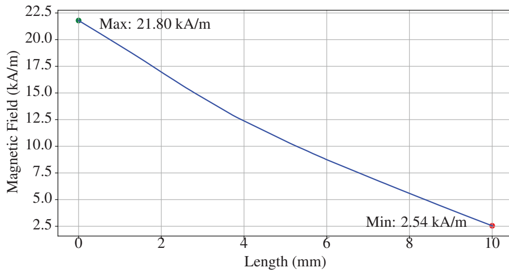
Figure 4: Magnetic field strength in the MRF for TPU wall thickness 0,2 mm
