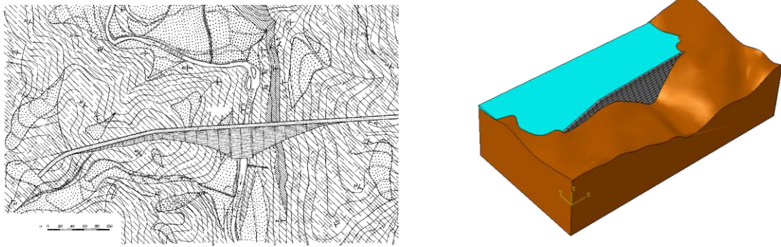
Figure 1: Dam drawing and FE model.
